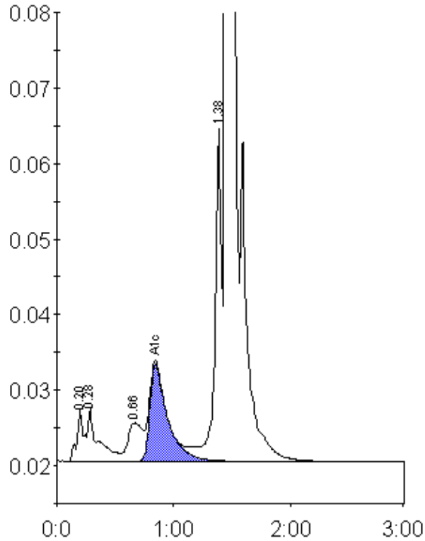
Peak table - ID: 10425835
